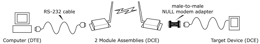
Figure B-06. Example of a Digi Radio Modem (DCE Device) connecting to another DCE device
