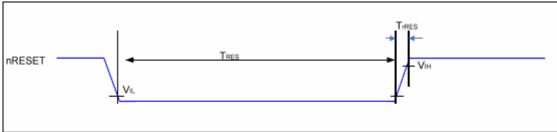
Fig. 14.4 Reset timing
